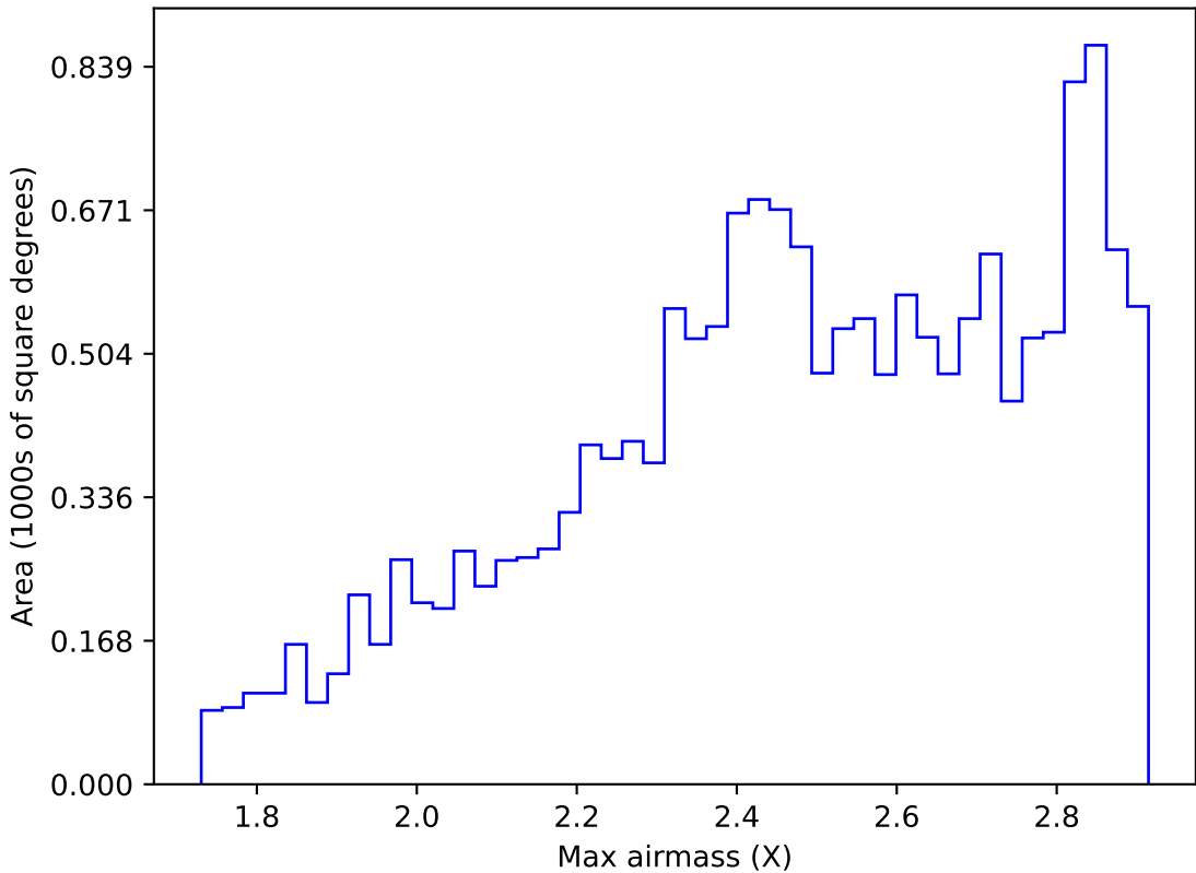
ddf_acor_sf15_lsf40_lsr50_v3.4_10yrs WFD i band: Max airmass
