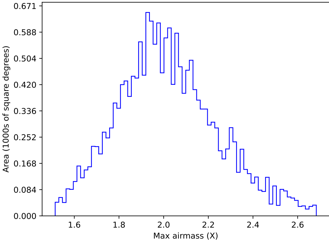
ddf_acor_sf15_lsf40_lsr50_v3.4_10yrs WFD g band: Max airmass
