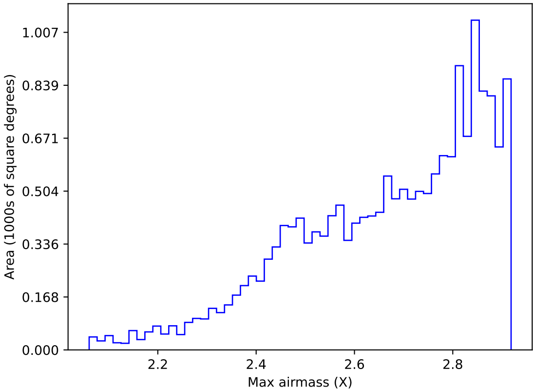
ddf_acor_sf15_lsf40_lsr50_v3.4_10yrs WFD all bands: Max airmass
