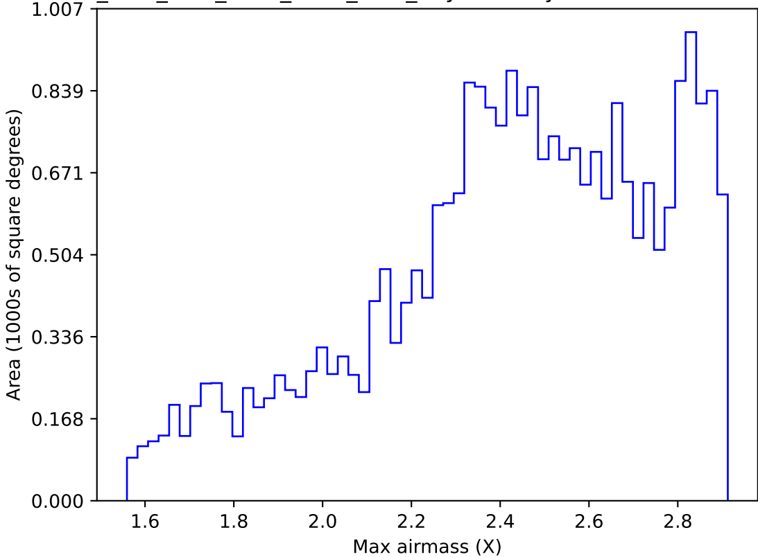
ddf_acor_sf15_lsf40_lsr50_v3.4_10yrs All sky z band: Max airmass
