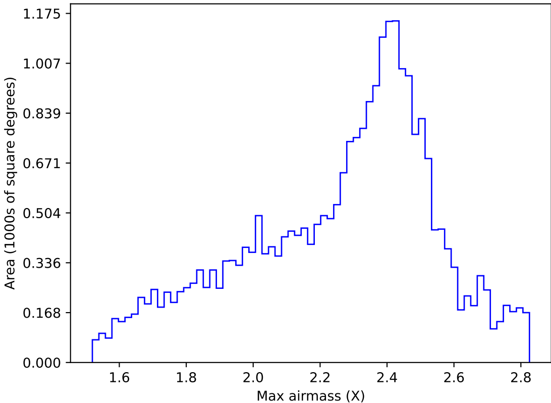
ddf_acor_sf15_lsf40_lsr50_v3.4_10yrs All sky r band: Max airmass
