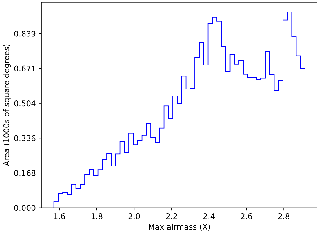
ddf_acor_sf15_lsf40_lsr50_v3.4_10yrs All sky i band: Max airmass
