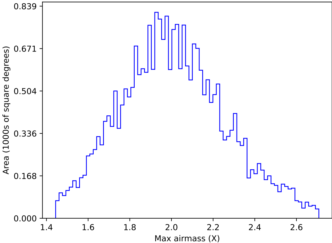
ddf_acor_sf15_lsf40_lsr50_v3.4_10yrs All sky g band: Max airmass
