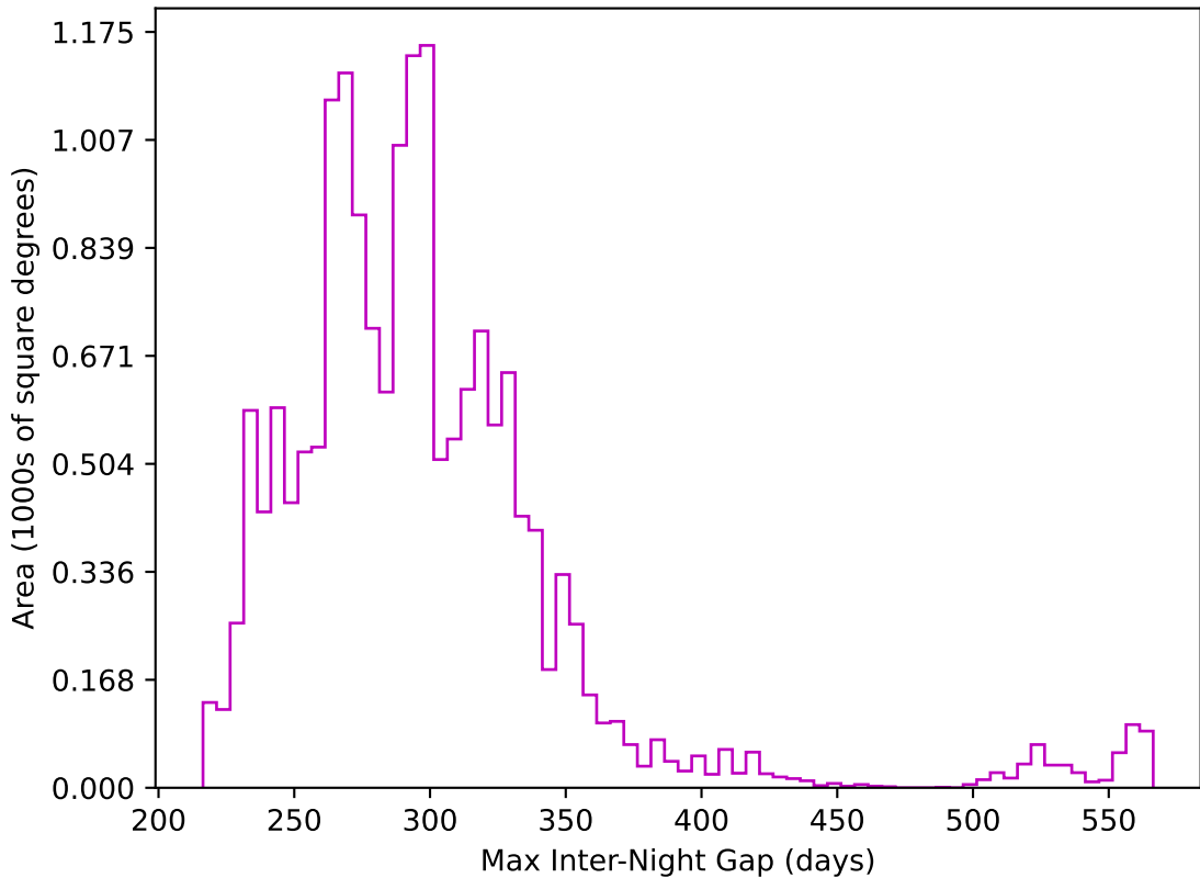
ddf_acor_sf15_lsf40_lsr50_v3.4_10yrs WFD z band: Max Inter-Night Gap
