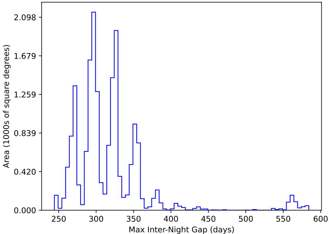
ddf_acor_sf15_lsf40_lsr50_v3.4_10yrs WFD y band: Max Inter-Night Gap
