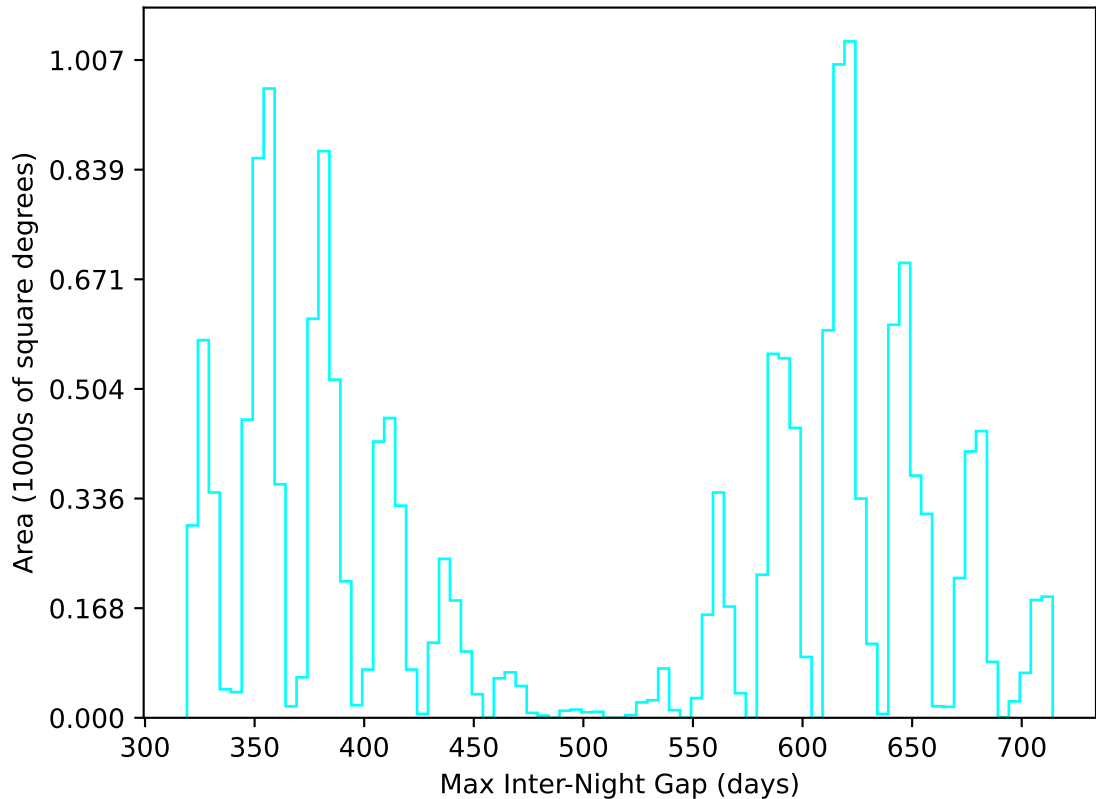
ddf_acor_sf15_lsf40_lsr50_v3.4_10yrs WFD u band: Max Inter-Night Gap
