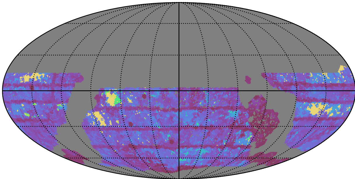
ddf_acor_sf15_lsf40_lsr50_v3.4_10yrs WFD r band: Max Inter-Night Gap
