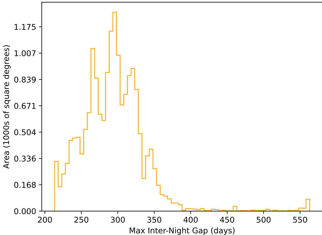
ddf_acor_sf15_lsf40_lsr50_v3.4_10yrs WFD r band: Max Inter-Night Gap
