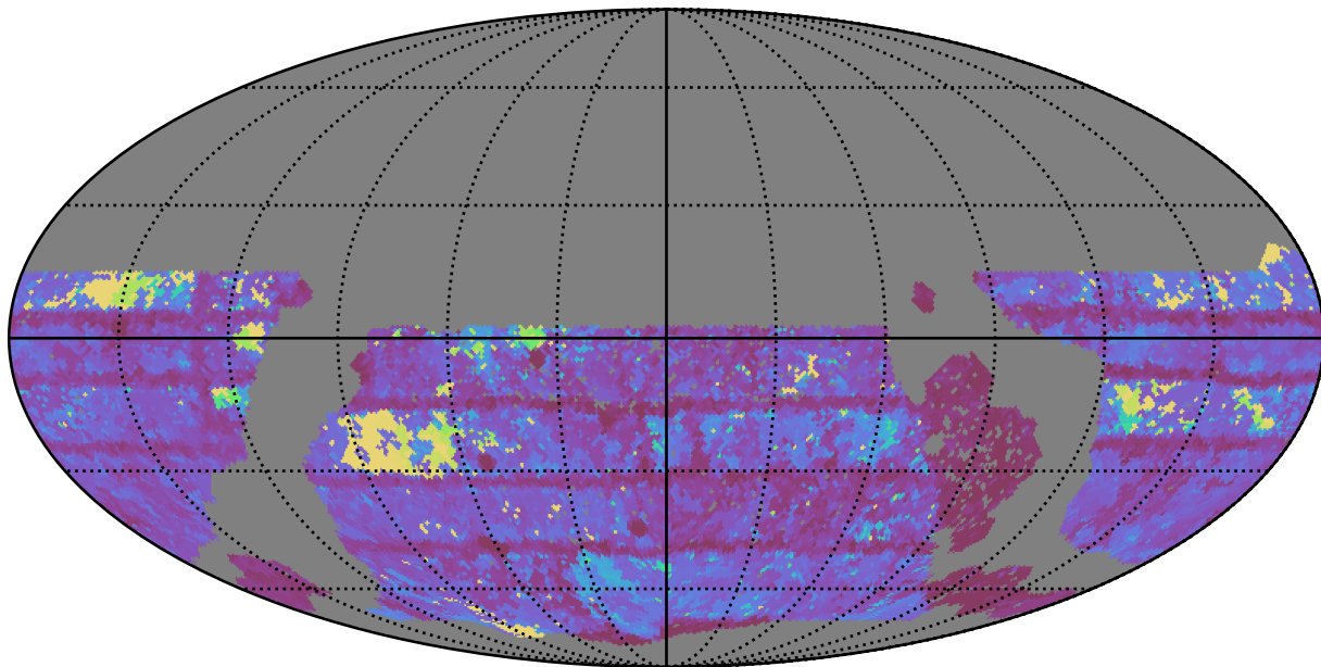
ddf_acor_sf15_lsf40_lsr50_v3.4_10yrs WFD i band: Max Inter-Night Gap
