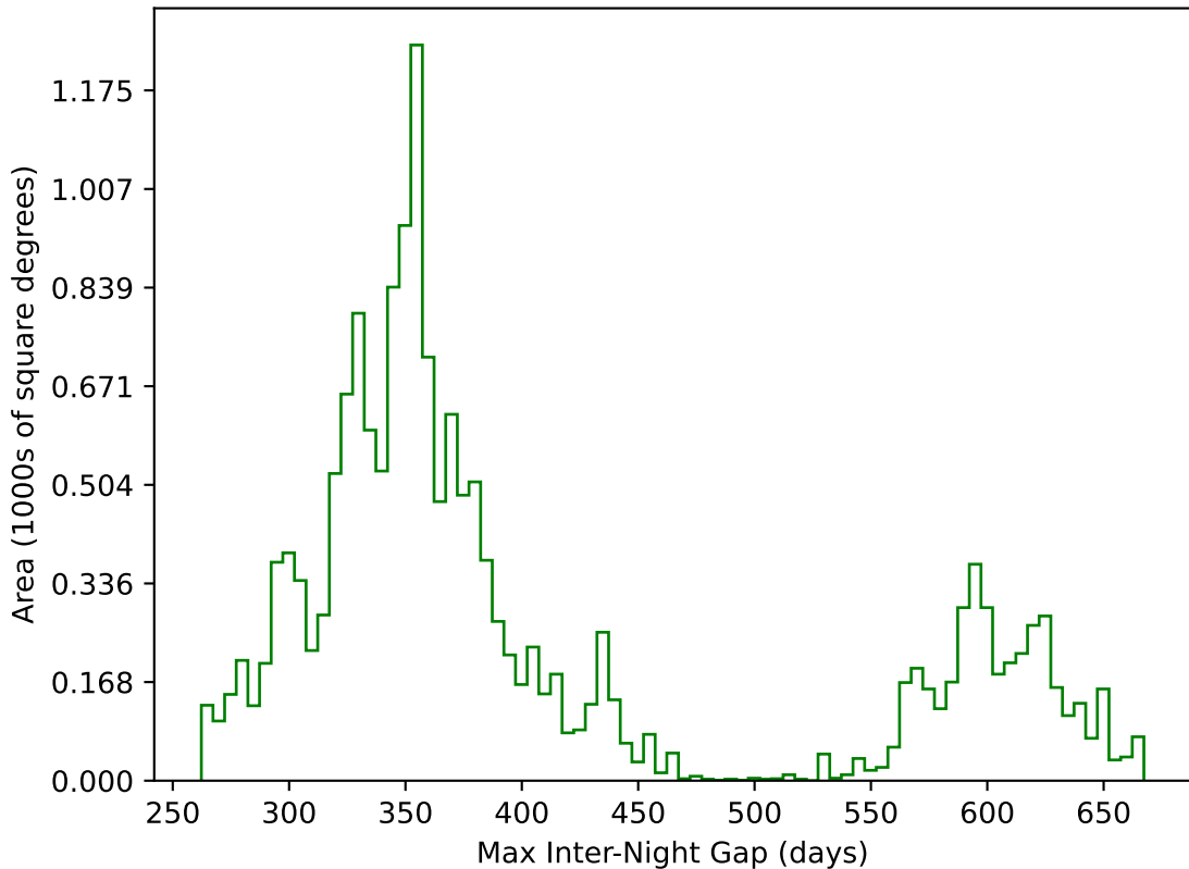
ddf_acor_sf15_lsf40_lsr50_v3.4_10yrs WFD g band: Max Inter-Night Gap
