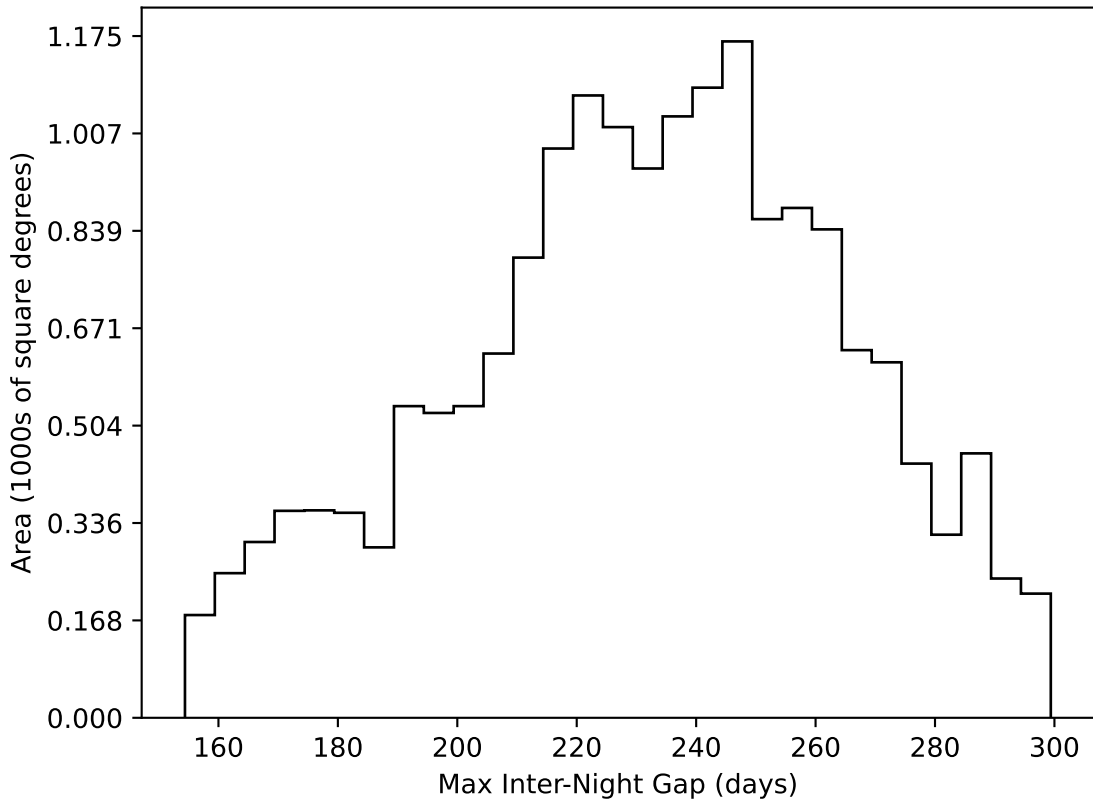
ddf_acor_sf15_lsf40_lsr50_v3.4_10yrs WFD all bands: Max Inter-Night Gap
