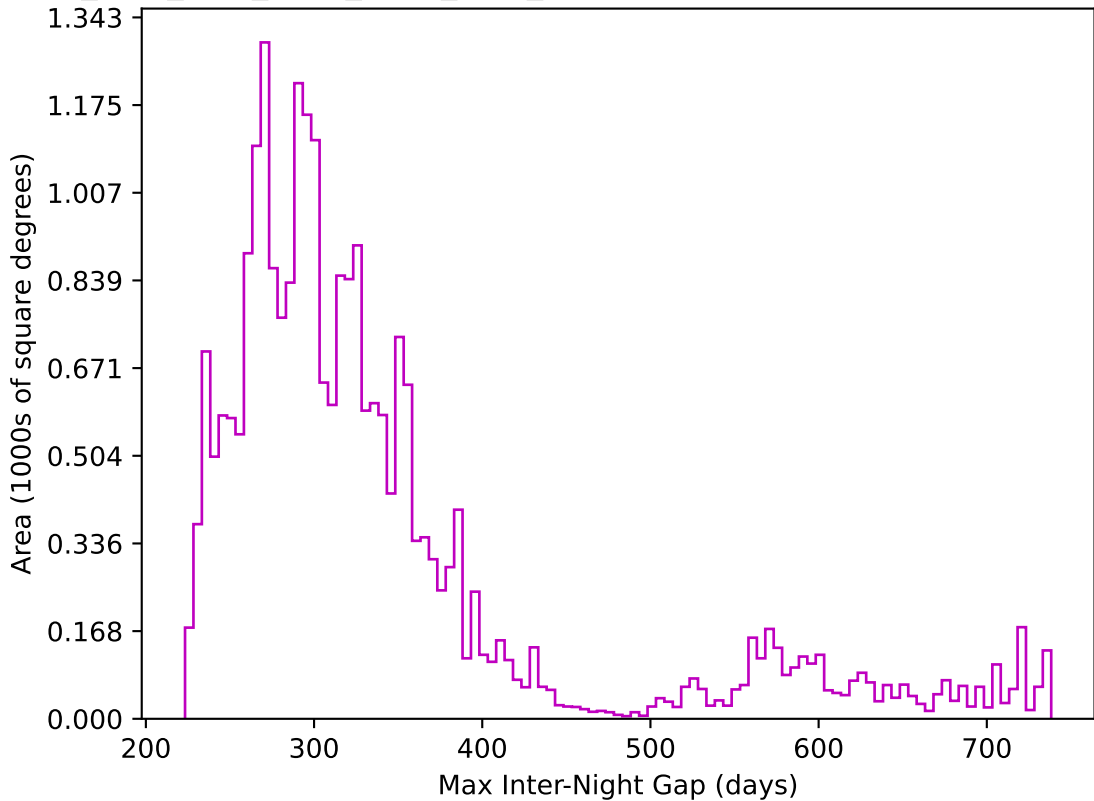
ddf_acor_sf15_lsf40_lsr50_v3.4_10yrs All sky z band: Max Inter-Night Gap
