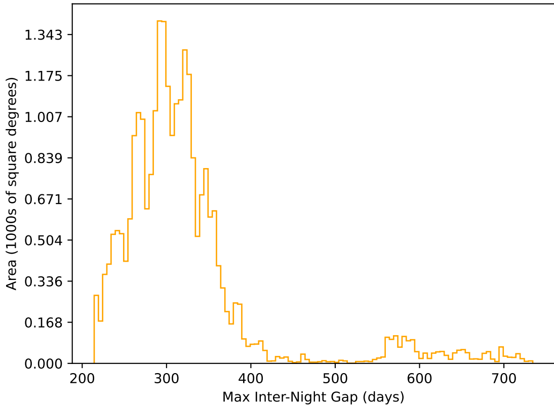
ddf_acor_sf15_lsf40_lsr50_v3.4_10yrs All sky r band: Max Inter-Night Gap
