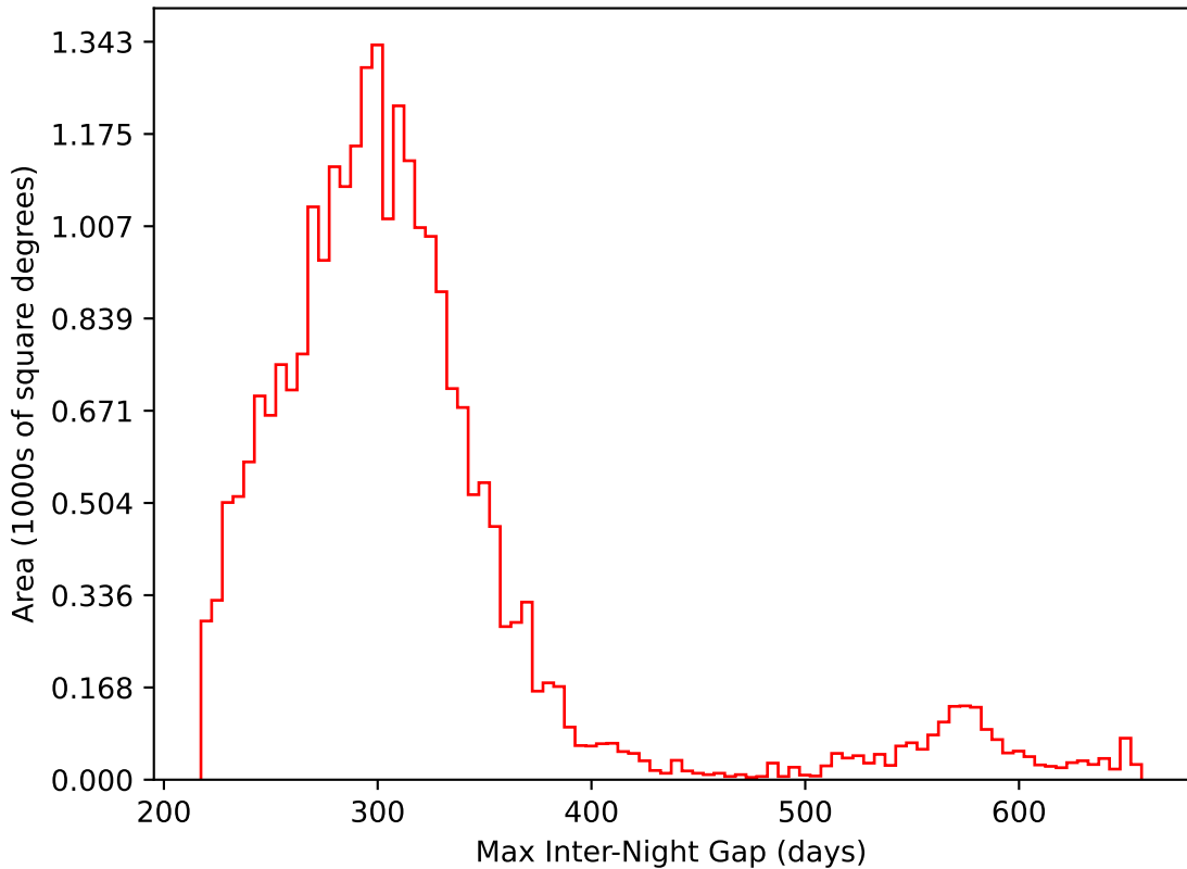
ddf_acor_sf15_lsf40_lsr50_v3.4_10yrs All sky i band: Max Inter-Night Gap
