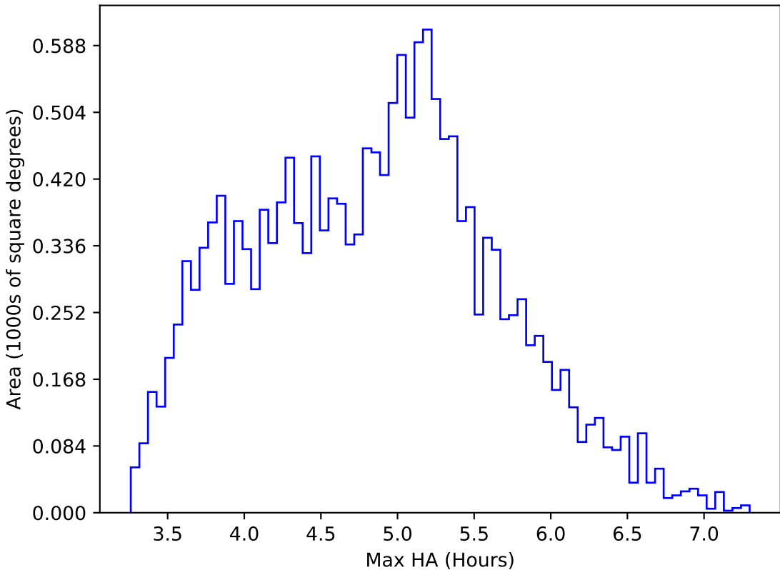
ddf_acor_sf15_lsf40_lsr50_v3.4_10yrs WFD z band: Max HA
