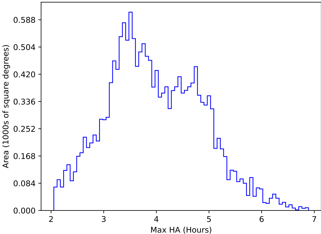
ddf_acor_sf15_lsf40_lsr50_v3.4_10yrs WFD u band: Max HA
