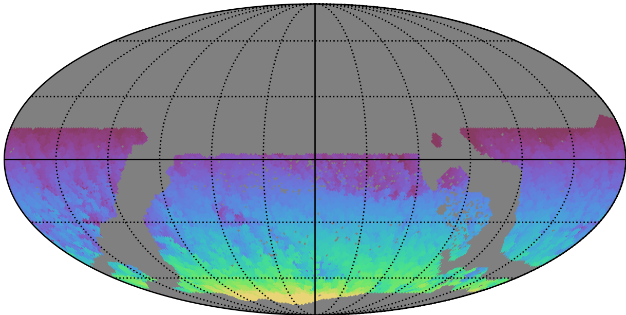
ddf_acor_sf15_lsf40_lsr50_v3.4_10yrs WFD all bands: Max HA
