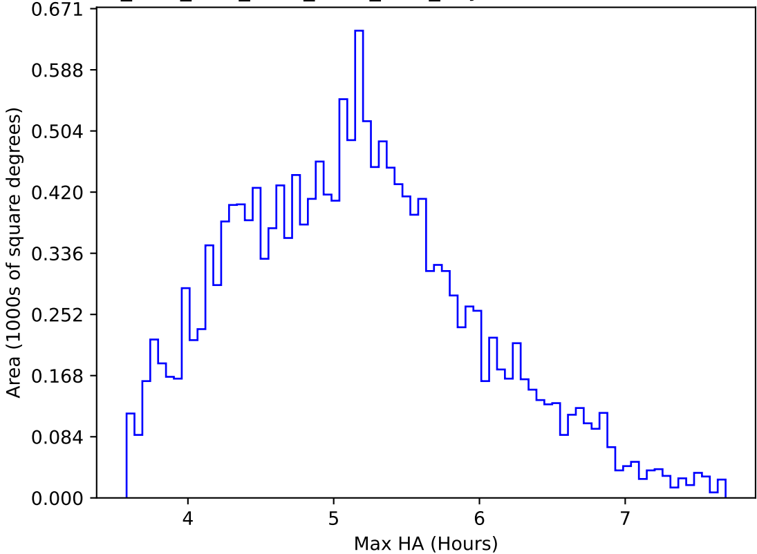
ddf_acor_sf15_lsf40_lsr50_v3.4_10yrs WFD all bands: Max HA
