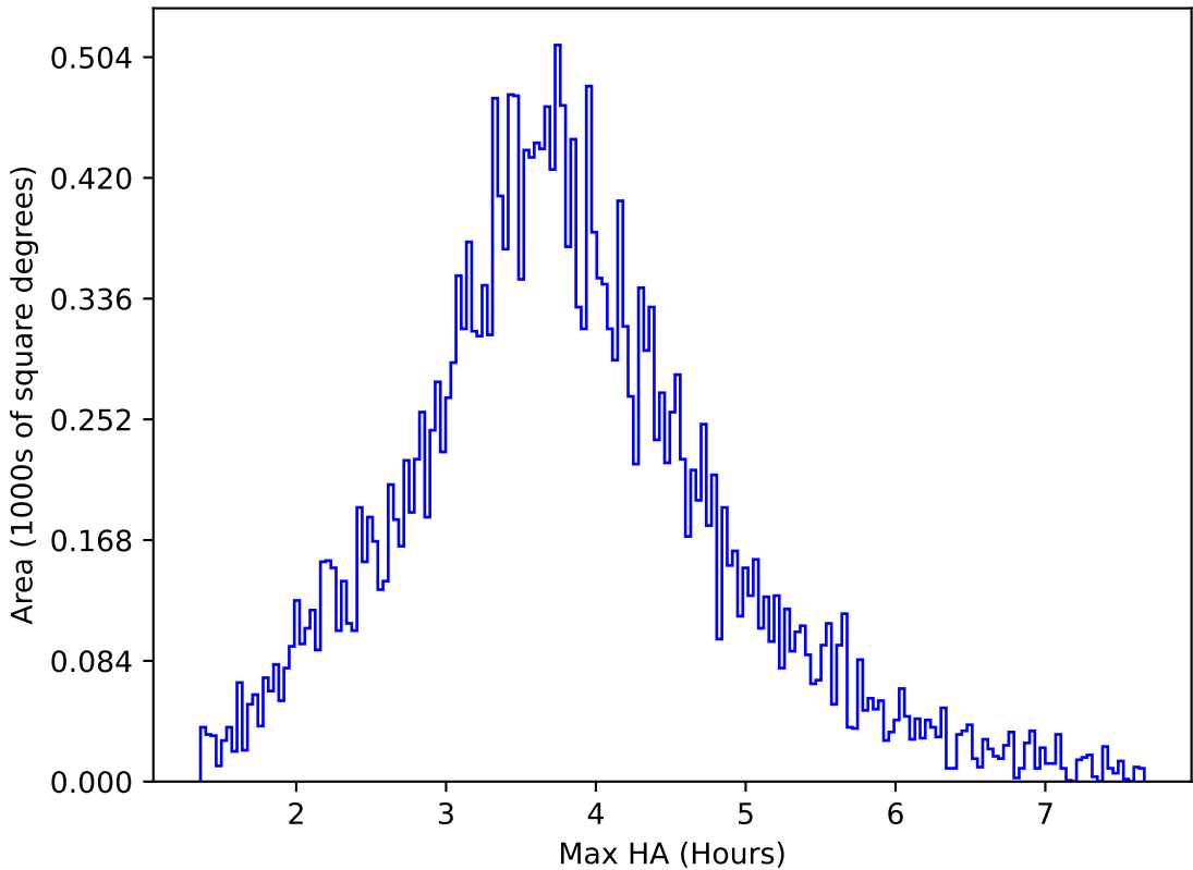
ddf_acor_sf15_lsf40_lsr50_v3.4_10yrs All sky g band: Max HA
