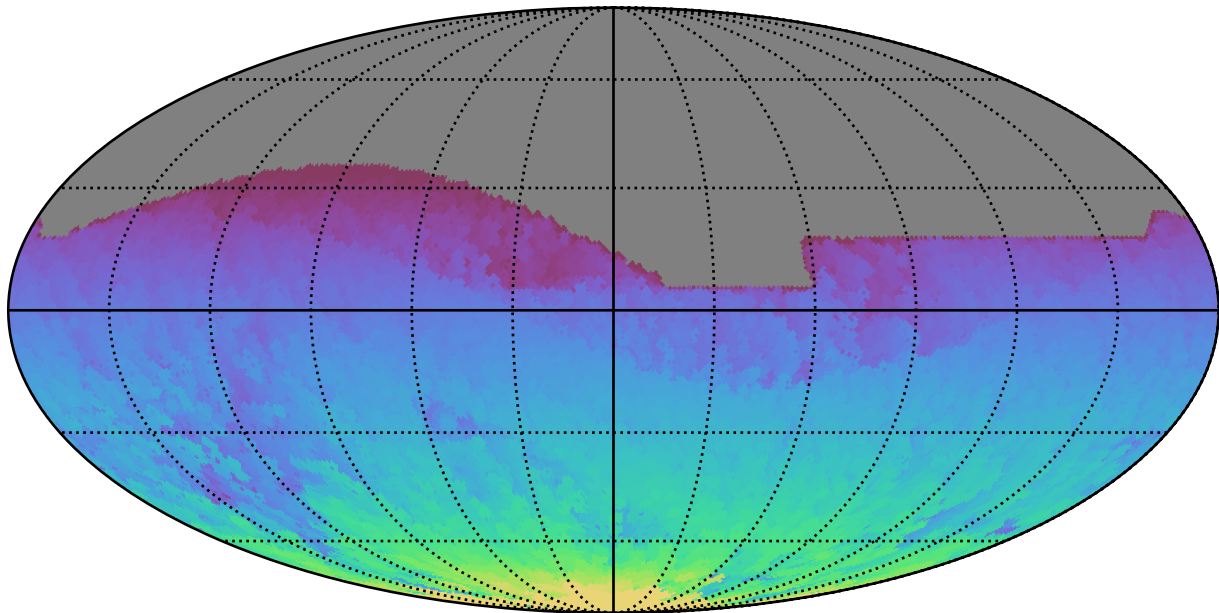
ddf_acor_sf15_lsf40_lsr50_v3.4_10yrs All sky all bands: Max HA
