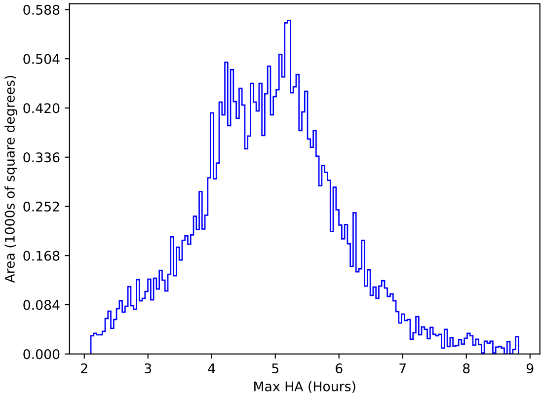
ddf_acor_sf15_ls40_lsr50_v3.4_10yrs All sky all bands: Max HA
