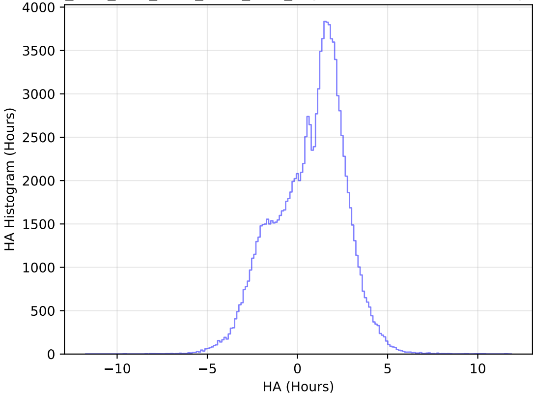
ddf_acor_sf15_lsf40_lsr50_v3.4_10yrs WFD u band: HA Histogram
