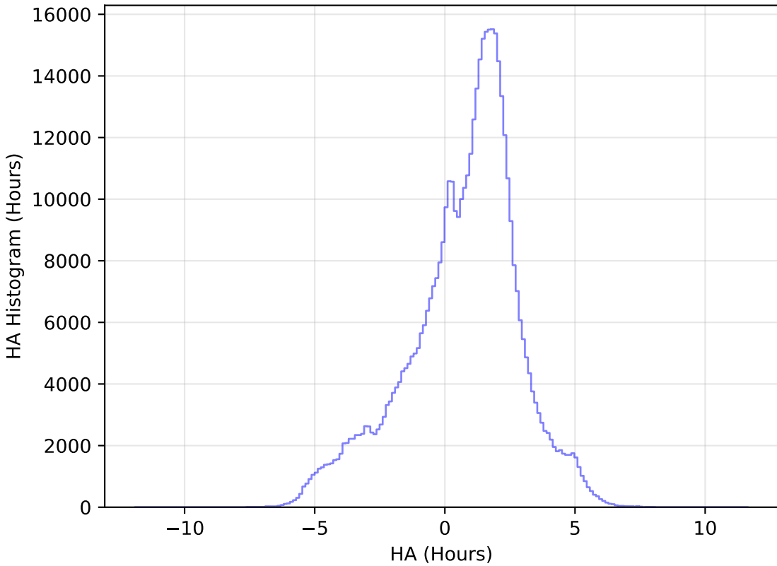
ddf_acor_sf15_lsf40_lsr50_v3.4_10yrs WFD i band: HA Histogram
