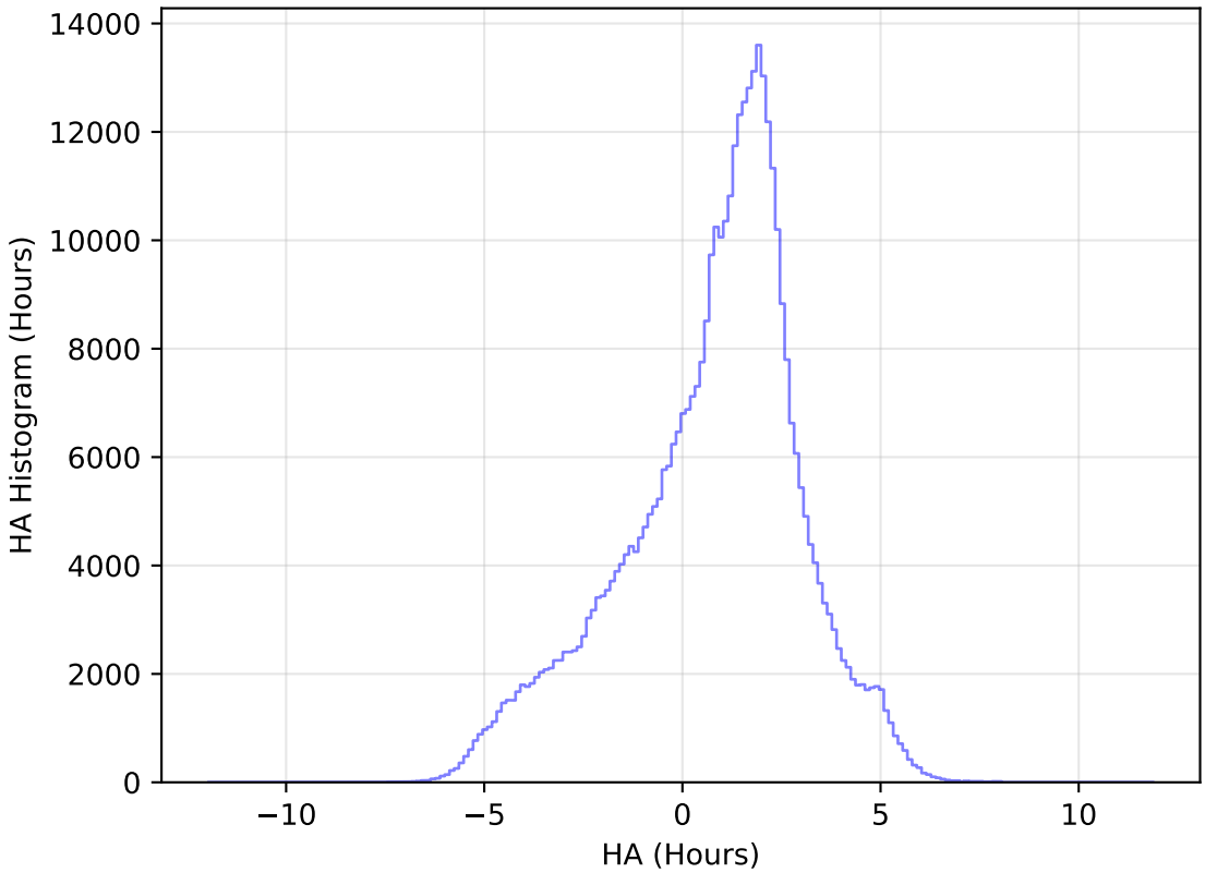
ddf_acor_sf15_lsf40_lsr50_v3.4_10yrs All sky z band: HA Histogram
