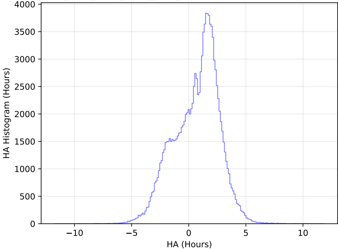
ddf_acor_sf15_lsf40_lsr50_v3.4_10yrs All sky u band: HA Histogram
