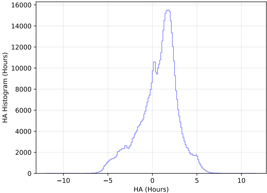
ddf_acor_sf15_lsf40_lsr50_v3.4_10yrs All sky i band: HA Histogram
