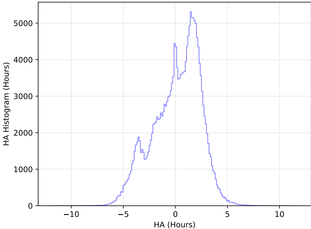
ddf_acor_sf15_lsf40_lsr50_v3.4_10yrs All sky g band: HA Histogram
