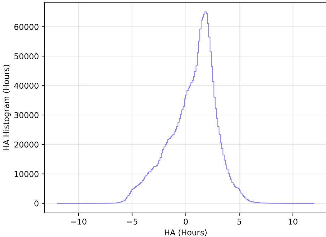
ddf_acor_sf15_lsf40_lsr50_v3.4_10yrs All sky all bands: HA Histogram
