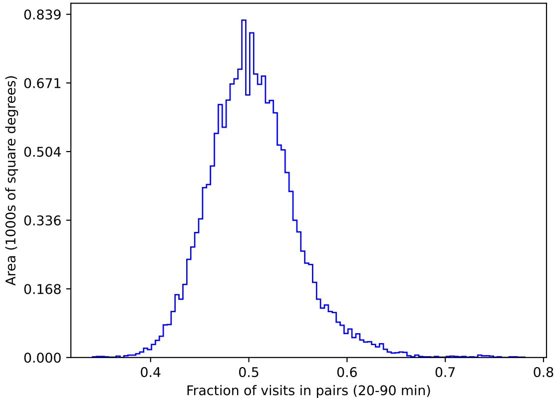
ddf_acor_sf15_lsf40_lsr50_v3.4_10yrs gri WFD: Fraction of visits in pairs (20-90 min)
