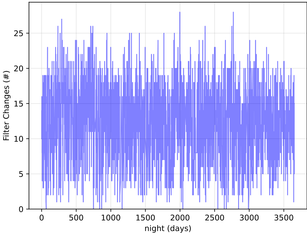
ddf_acor_sf15_lsf40_lsr50_v3.4_10yrs Per Night: Filter Changes
