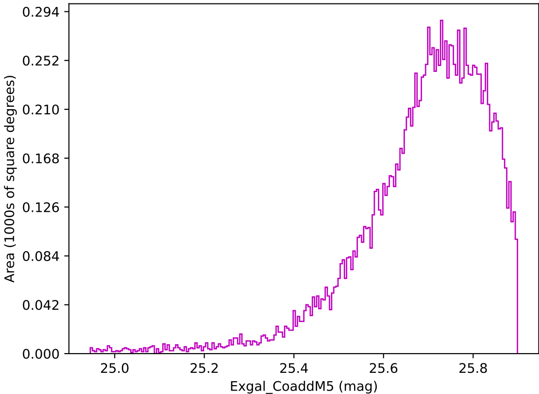
ddf_acor_sf15_lsf40_lsr50_v3.4_10yrs WFD z band: Exgal_CoaddM5
