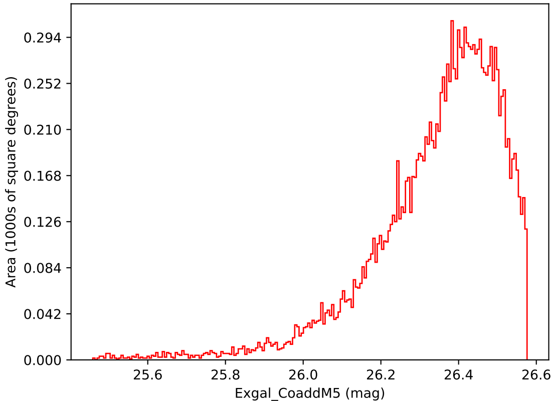
ddf_acor_sf15_lsf40_lsr50_v3.4_10yrs WFD i band: Exgal_CoaddM5
