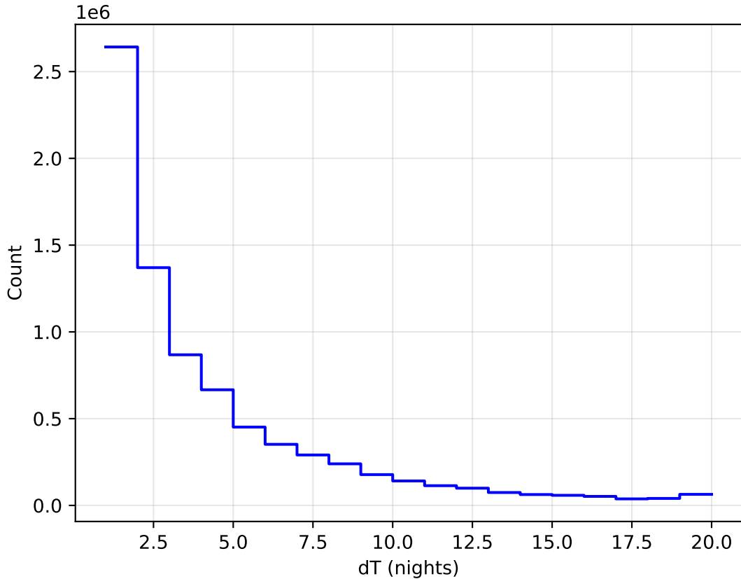
ddf_acor_sf15_lsf40_lsr50_v3.4_10yrs WFD all bands: DeltaNight Histogram
