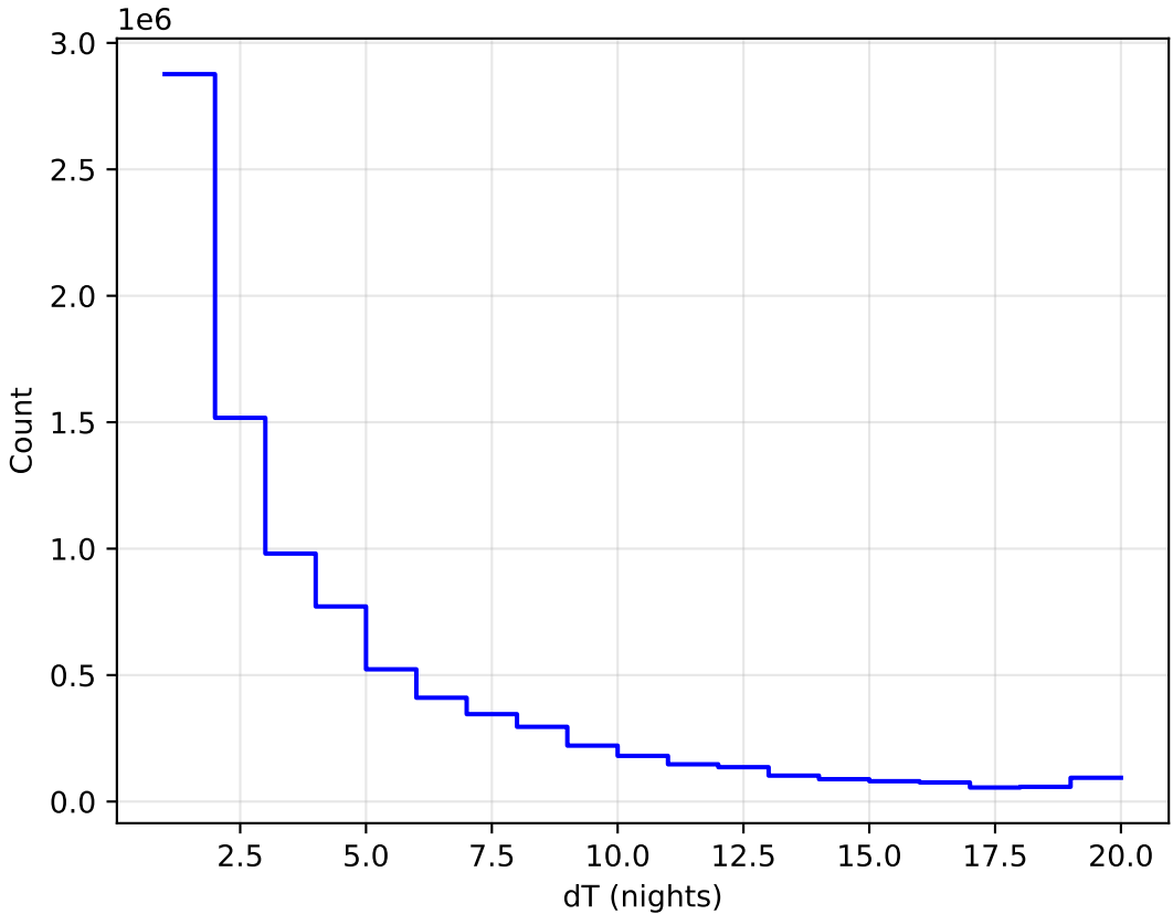
ddf_acor_sf15_lsf40_lsr50_v3.4_10yrs All sky all bands: DeltaNight Histogram
