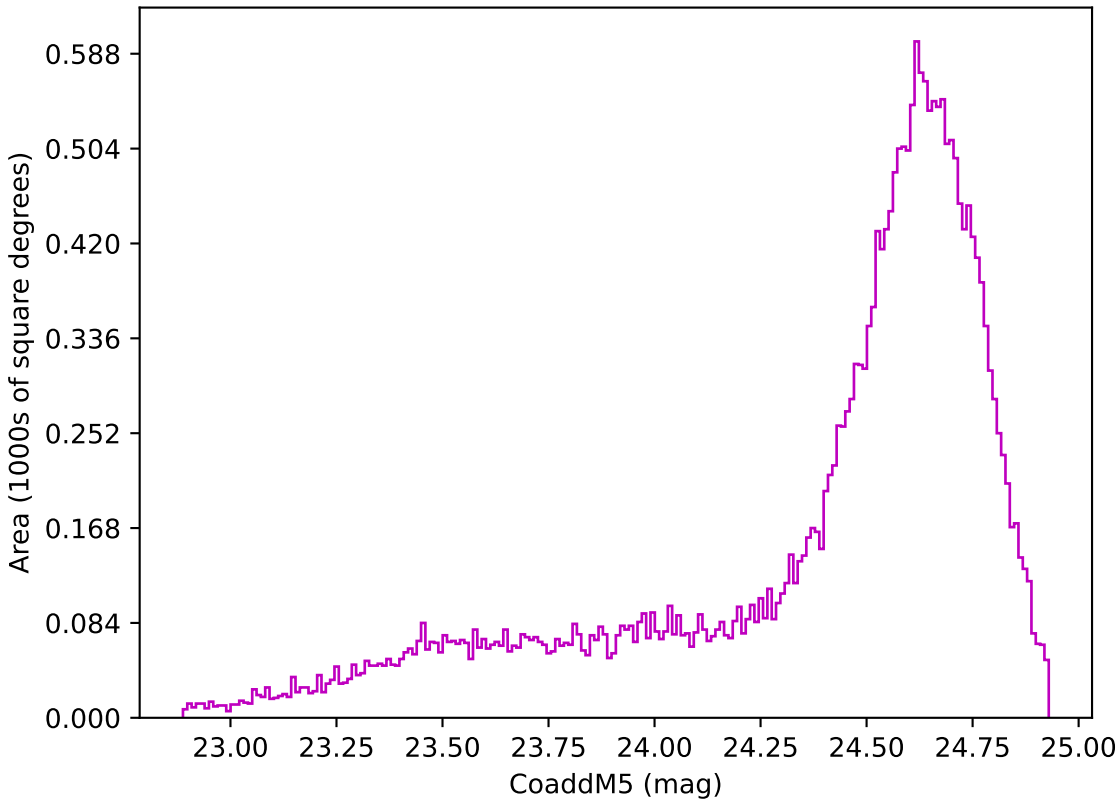
ddf_acor_sf15_lsf40_lsr50_v3.4_10yrs Yr 1 z band: CoaddM5
