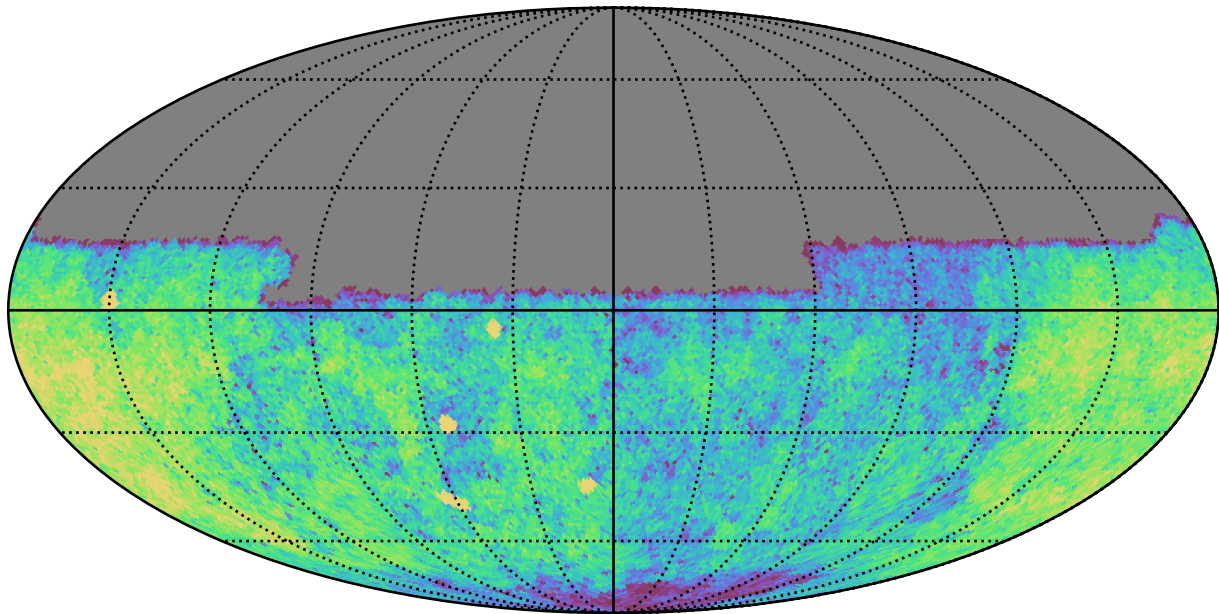
ddf_acor_sf15_lsf40_lsr50_v3.4_10yrs Yr 1 u band: CoaddM5
