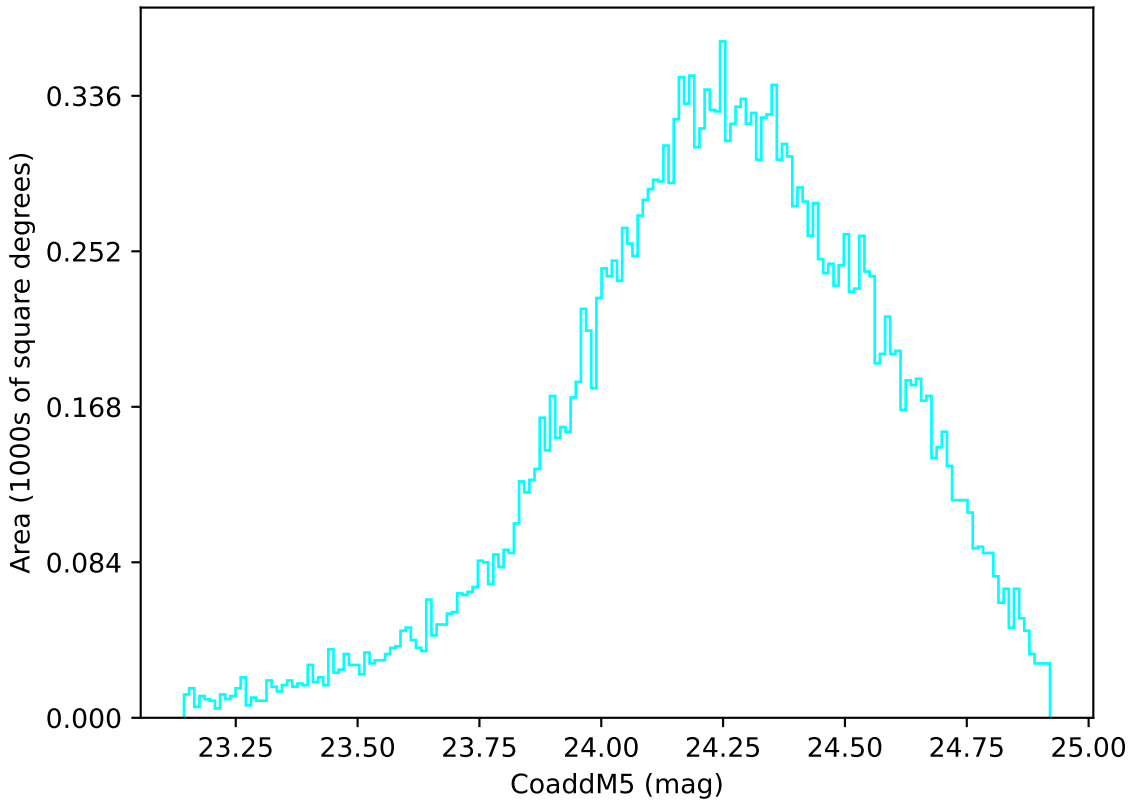
ddf_acor_sf15_lsf40_lsr50_v3.4_10yrs Yr 1 u band: CoaddM5
