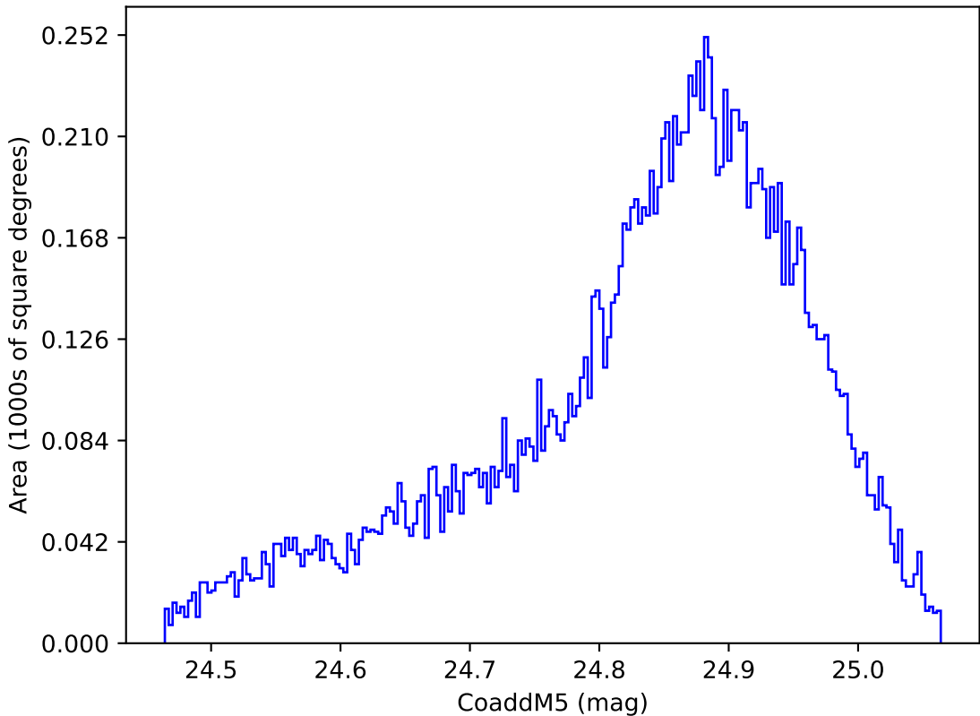
ddf_acor_sf15_ls40_lsr50_v3.4_10yrs WFD y band: CoaddM5
