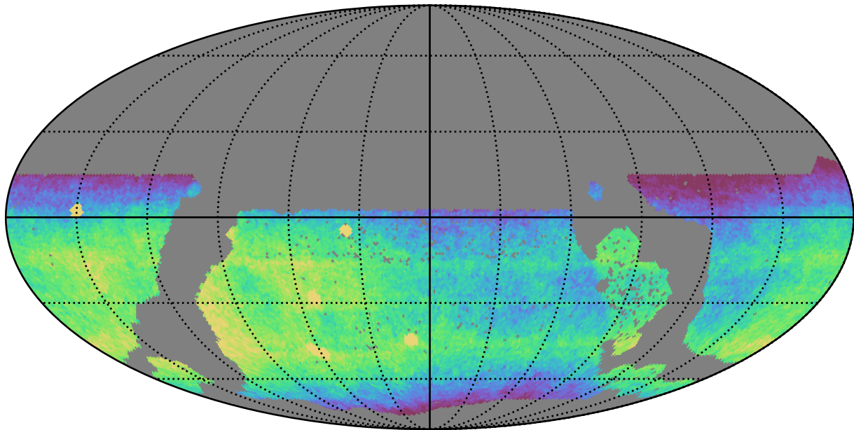
ddf_acor_sf15_lsf40_lsr50_v3.4_10yrs WFD r band: CoaddM5
