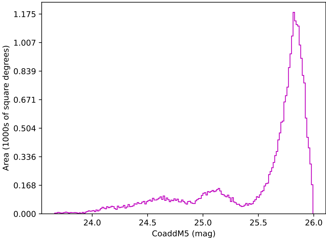
ddf_acor_sf15_lsf40_lsr50_v3.4_10yrs All sky z band: CoaddM5
