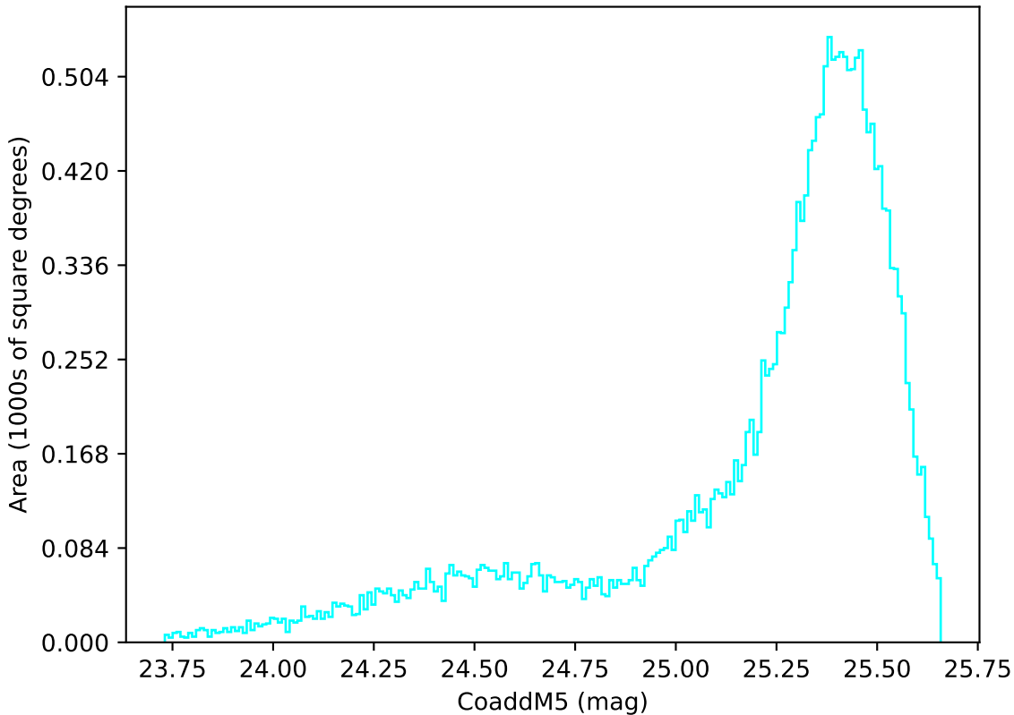
ddf_acor_sf15_lsf40_lsr50_v3.4_10yrs All sky u band: CoaddM5
