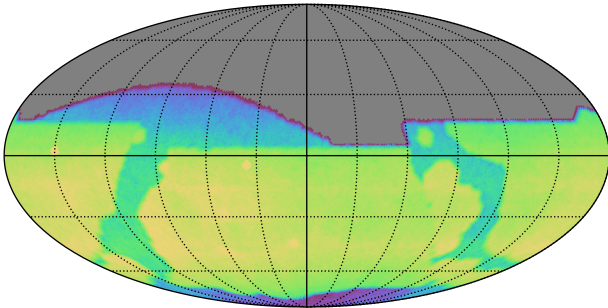
ddf_acor_sf15_lsf40_lsr50_v3.4_10yrs All sky r band: CoaddM5
