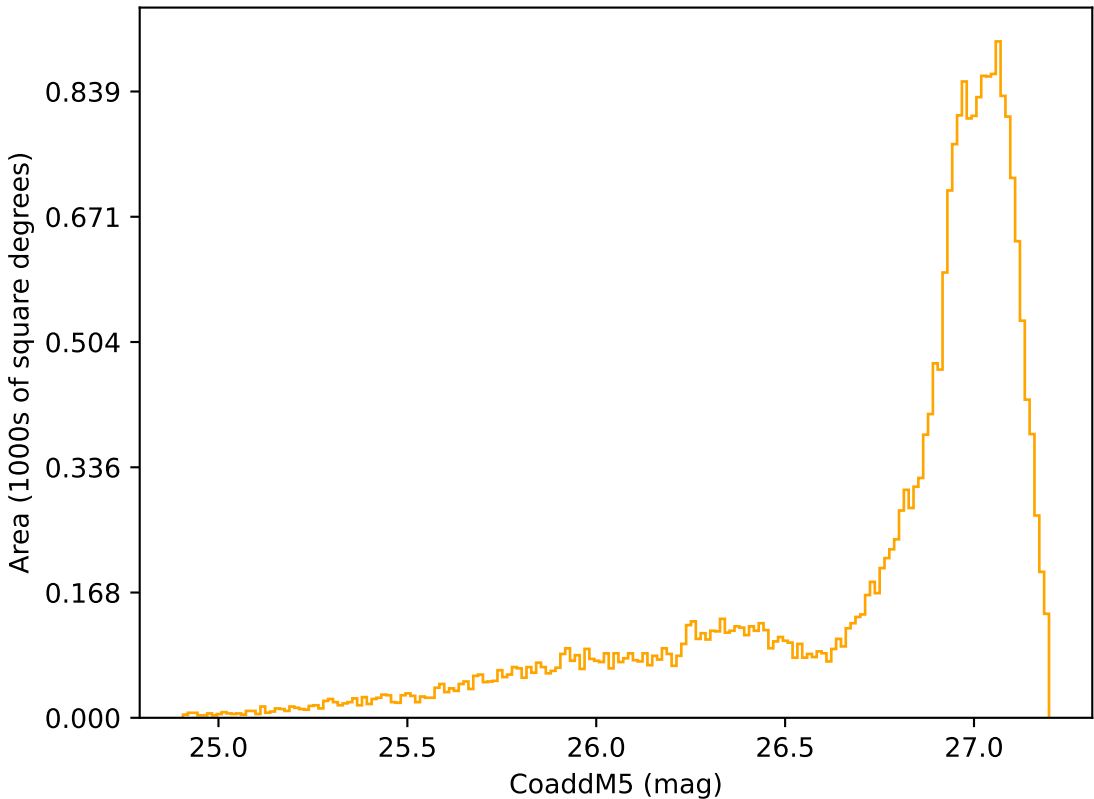
ddf_acor_sf15_lsf40_lsr50_v3.4_10yrs All sky r band: CoaddM5
