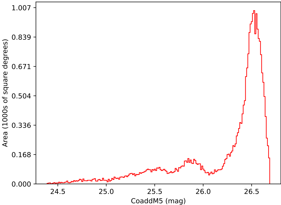
ddf_acor_sf15_lsf40_lsr50_v3.4_10yrs All sky i band: CoaddM5
