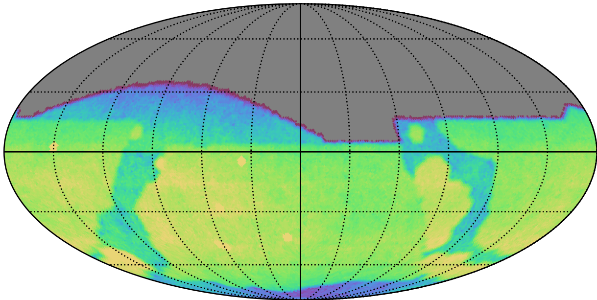
ddf_acor_sf15_lsf40_lsr50_v3.4_10yrs All sky g band: CoaddM5
