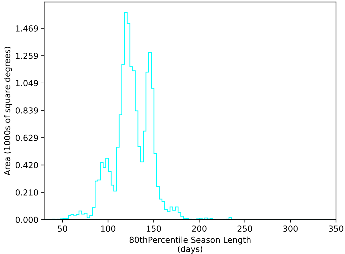
ddf_acor_sf15_lsf40_lsr50_v3.4_10yrs WFD u band: 80thPercentile Season Length
